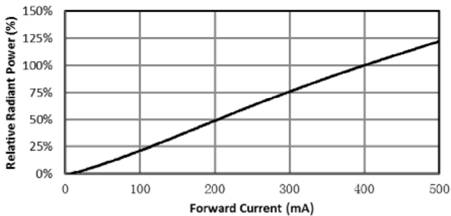
Relative Radiant Power vs. Forward Current ( T_a=25^\circ\text{C} )
