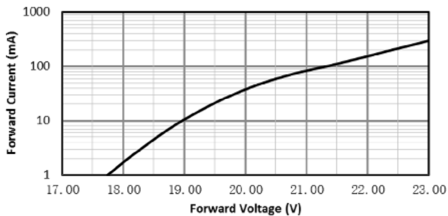
Forward Current vs. Forward Voltage ( T_a=25^\circ\text{C} )
